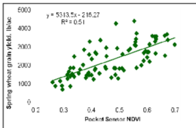
Figure 2. Relationship between Pocket Sensor NDVI and spring wheat grain yield, WTARC and WARC (combined locations), 2011.
